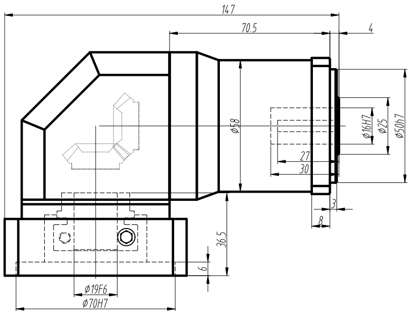
标准轴 Standard output shaft
